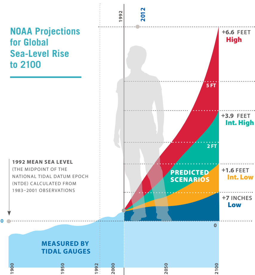
FIGURE 2.9: NOAA PROJECTIONS FOR GLOBAL SEA-LEVEL RISE TO 2100. THE LOWEST SCENARIO ASSUMES VERY MODERATE GLOBAL CLIMATE CHANGE AND A GENERAL CONTINUATION OF THE SEA-LEVEL RISE TREND OBSERVED IN THE 20TH CENTURY TIDE GAUGE RECORD. THE HIGHEST SCENARIO ASSUMES SIGNIFICANT GLOBAL CLIMATE CHANGE THAT INDUCES LARGE-SCALE MELTING OF THE GREENLAND AND ANTARCTIC ICE SHEETS.
